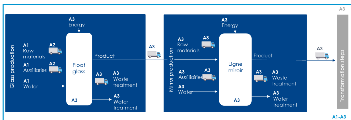
Figure 1 : Relevant LCA steps for MIRALITE®PURE. Steps in blue are declared in this EPD, steps in grey are not declared.
